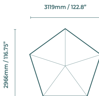
SKYLIGHT DIMENSIONS
