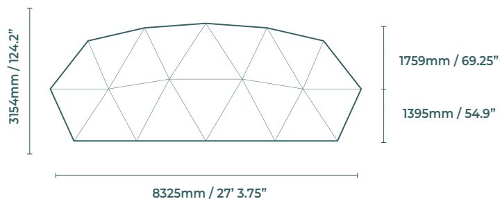
TEMPERED GLASS PANORAMIC STRUCTURE WINDOWS With Cover On
