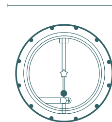
CIRCLE GLASS WINDOW (Operable with screen) 445mm / 17.5"
